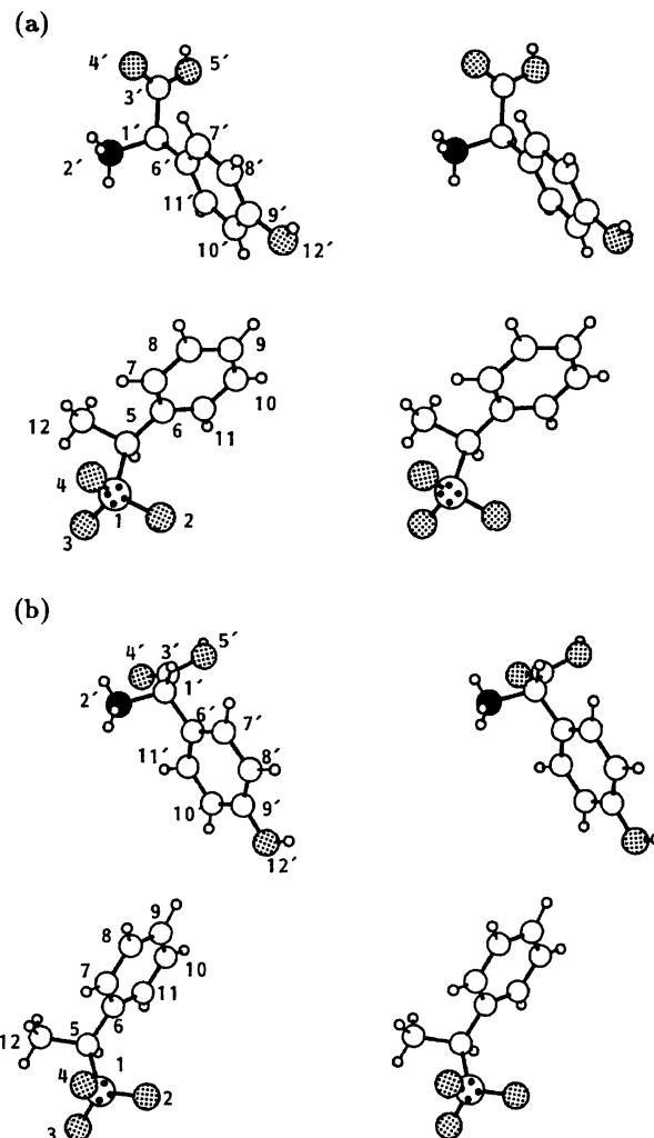
Fig. 1. Labeled stereoscopic drawings of diastereomeric salts. (a) D-HPG \cdot(-) -PES; (b) L-HPG \cdot(-) -PES. H, \circ ; C, \circ ; O, \bullet ; N, \bullet ; S, \oplus .
